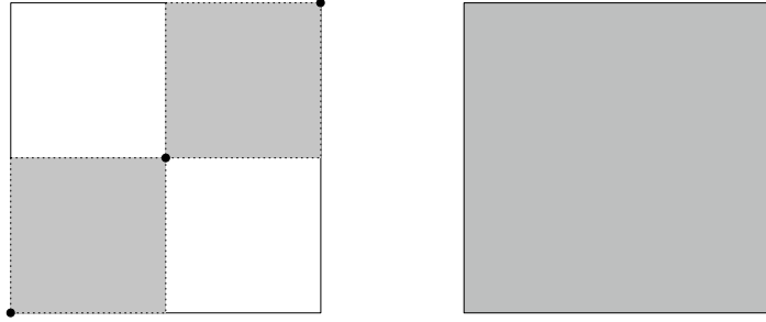
FIGURE 2.1. The graph of the equivalence relation from §2.2 and its transitive-closure.
