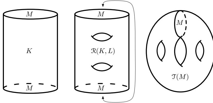
FIGURE 3. The construction of the hyperbolized mapping torus \mathcal{J}(M) .
