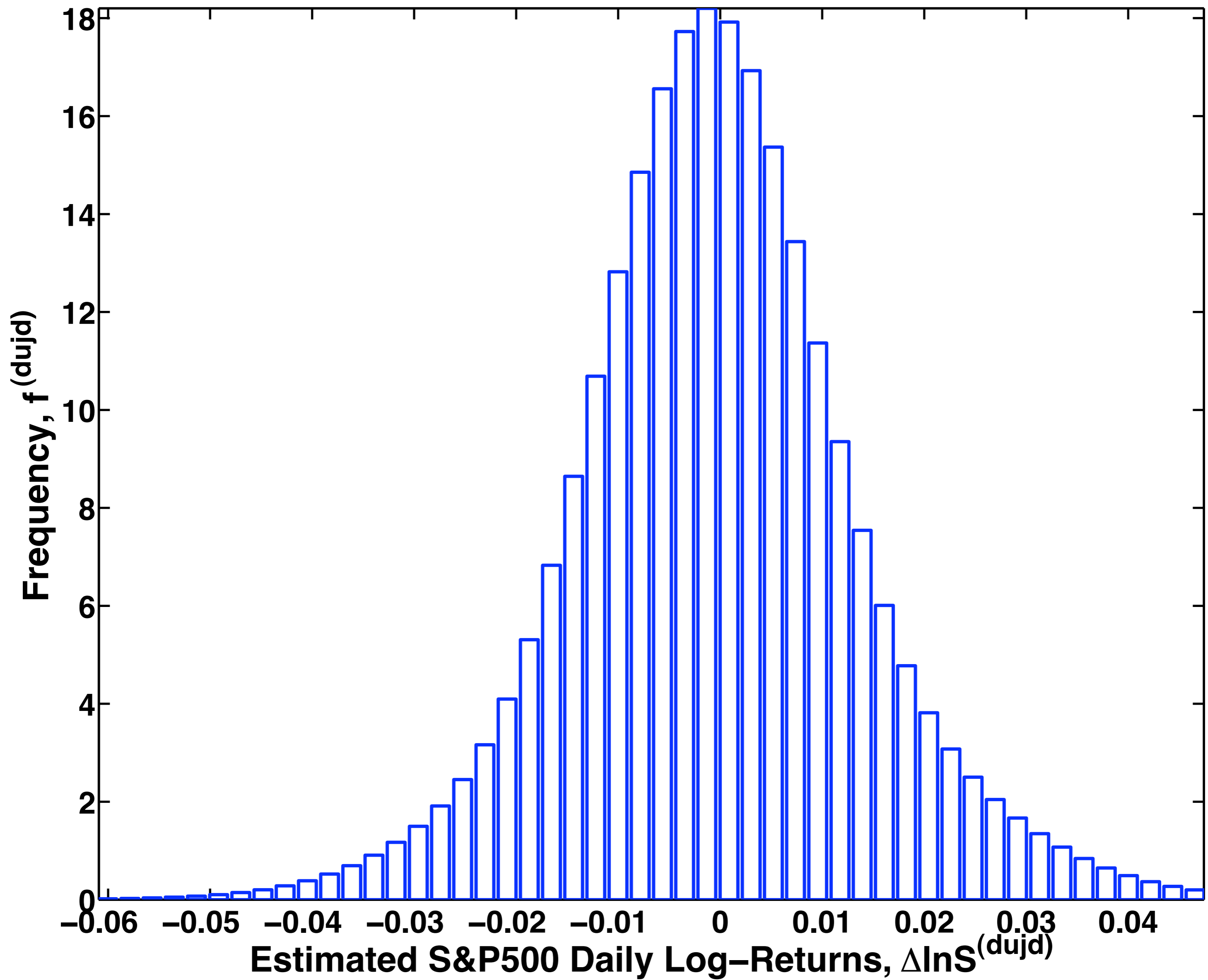
Histogram: Fitted Daily Log-Returns, Year 2000
