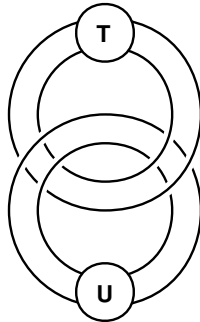
Fig. 1: The diagram H(T, U)
