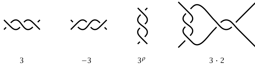
Fig. 2: Examples of tangles
