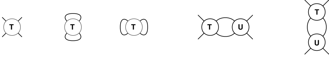
Fig. 3: A tangle T , its closures T^N , T^D and the tangle combinations T + U , T * U
