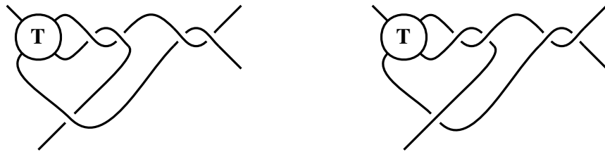
Fig.5: The tangles T^\omega, T^{\bar{\omega}}
