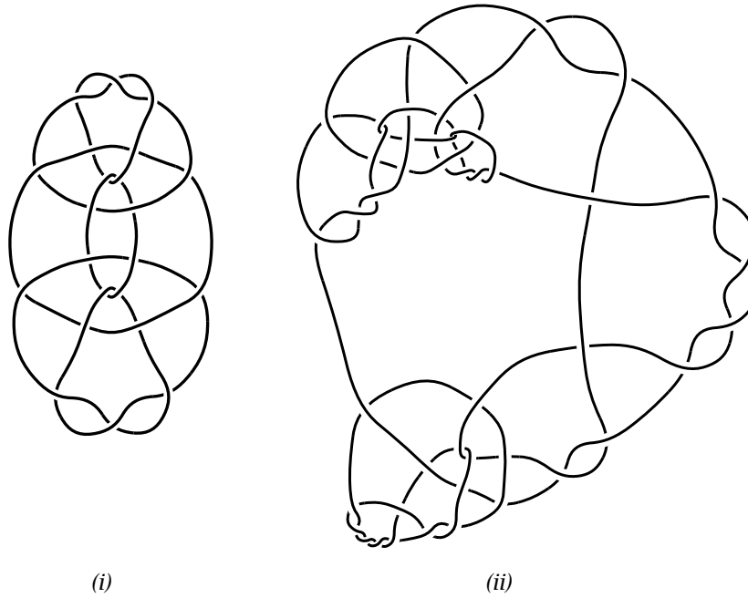
Fig. 10: Prime 4- and 5-component links with trivial Jones polynomial
